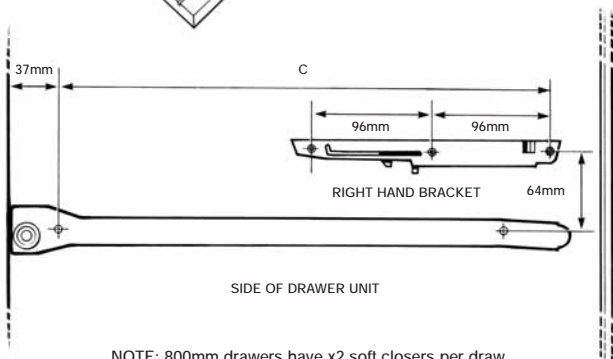
RUNNER DIAGRAM
